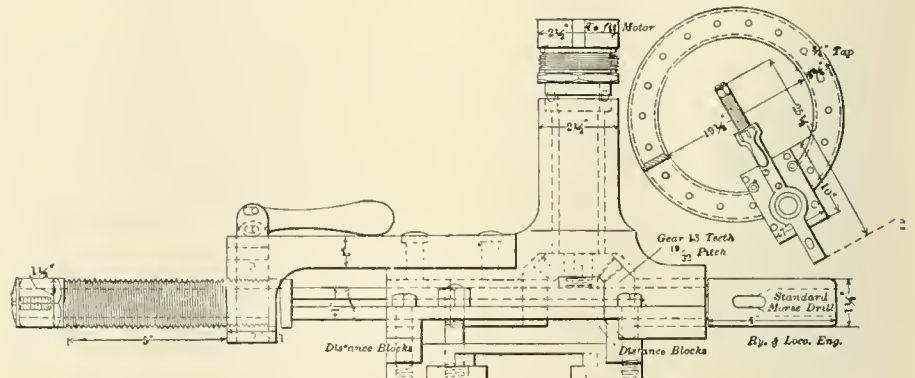
FIGS. 1 AND 2.—SECTIONAL VIEW OF RIGHT-ANGLED DRILL.
